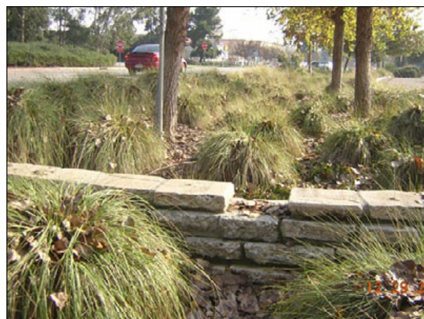
Figure C-27. Stacked concrete check dam.
