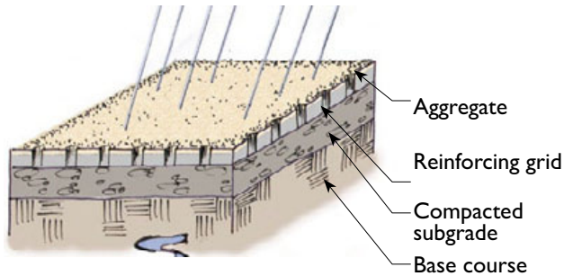
Figure 49. Reinforced gravel paving profile.
