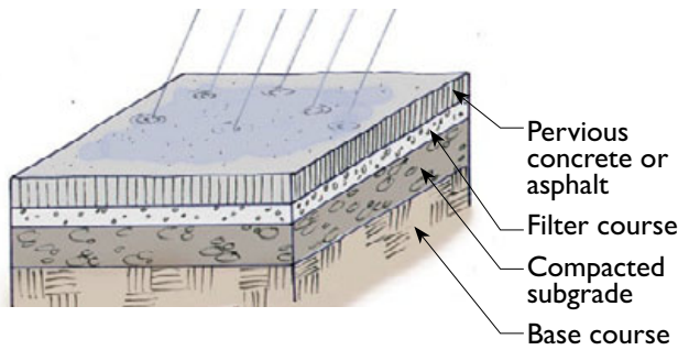
Figure 42. Pervious concrete profile.
