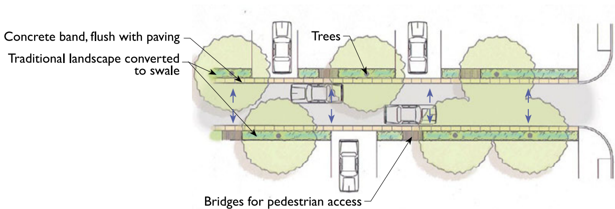
Figure 79. Side swales—plan view.
