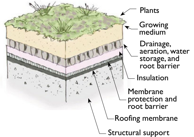
Figure 66. Green roof profile.
